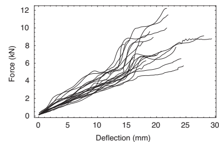
Figure 6. Force-deflection responses from all cadaver knee/femur response tests conducted using molded-knee interfaces at a 1.2-m/s platform velocity.
