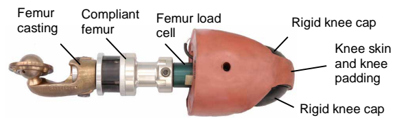
Figure 2. THOR knee/femur complex with Hybrid III upper femur casting.
