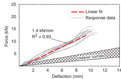
Figure 11. Force-deflection responses for loading of THOR knee/femur complex by a molded-knee interface at a 1.2-m/s platform velocity relative to the new cadaver response corridor.
