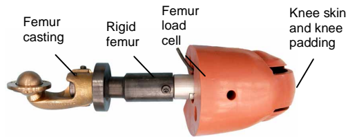
Figure 1. Hybrid III knee/femur complex.
