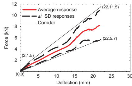
Figure 7. Mean and \pm 1 SD knee/femur force-deflection responses and corridor developed from cadaver responses to molded-knee interface loading at a 1.2-m/s platform velocity.
